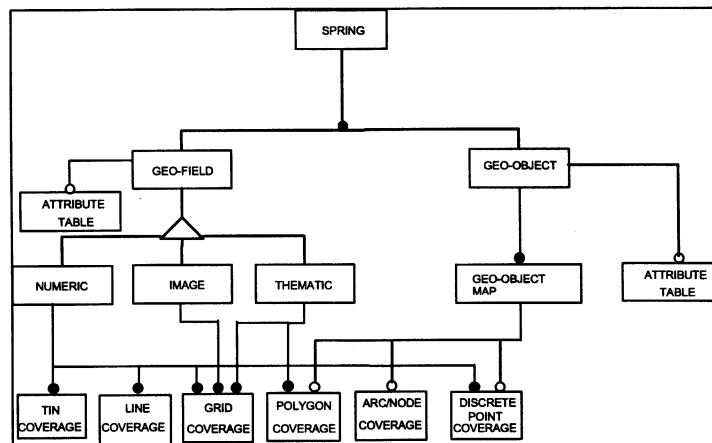
Fig. 3. SPRING's data model.
