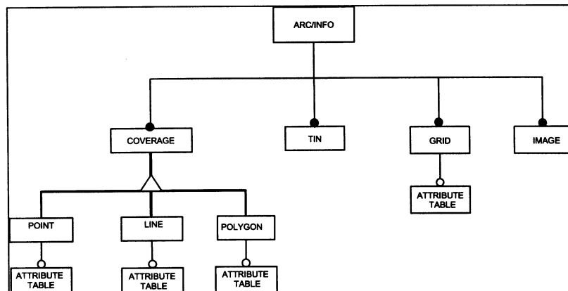
Fig. 2. ARC/INFO's data model.
