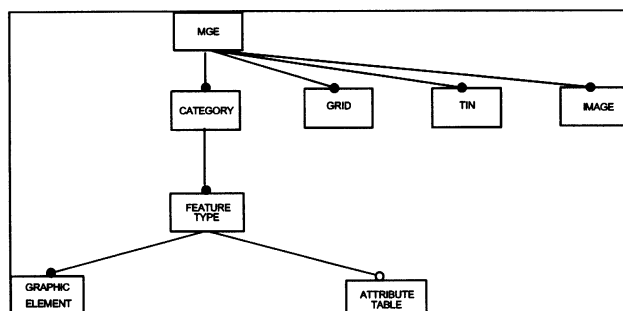
Fig. 1. MGE's data model
