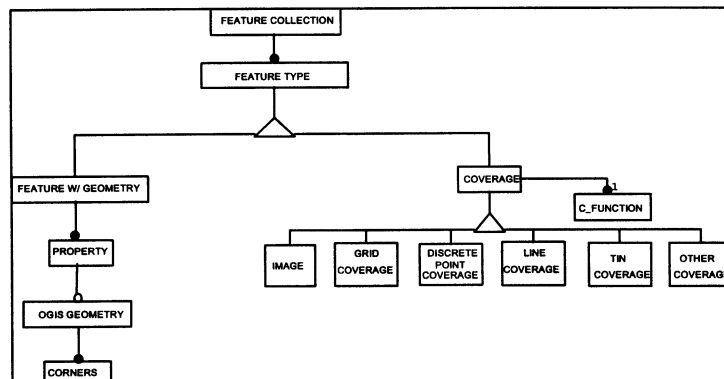
Fig. 4. OpenGIS data model.
